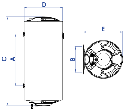
Vertical type
