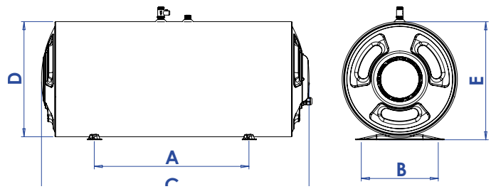
Floor type
