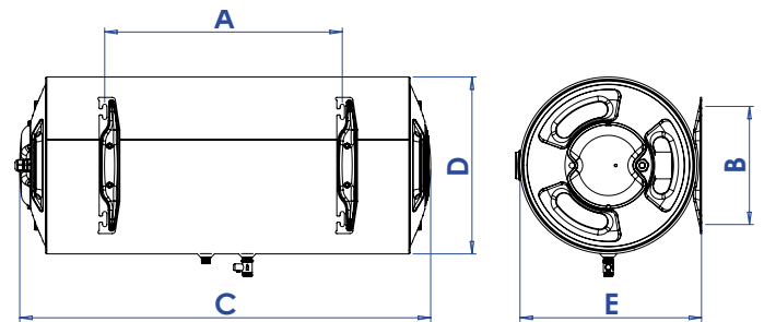
Horizontal type
